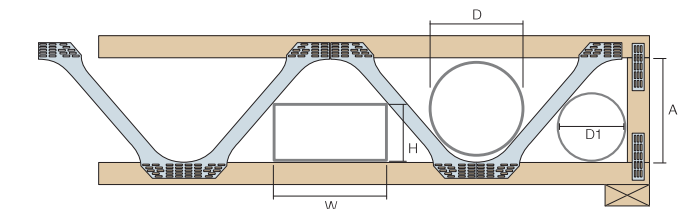
Technical Specification Joist depth (in mm) 195, 219, 254, 304, 417
